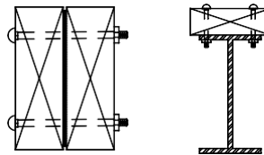
WOOD-TO-METAL CONNECTIONS
